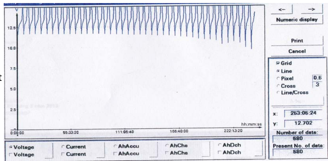
New Battery #3 W/O SRS fails at 253 hours (41 cycles)
