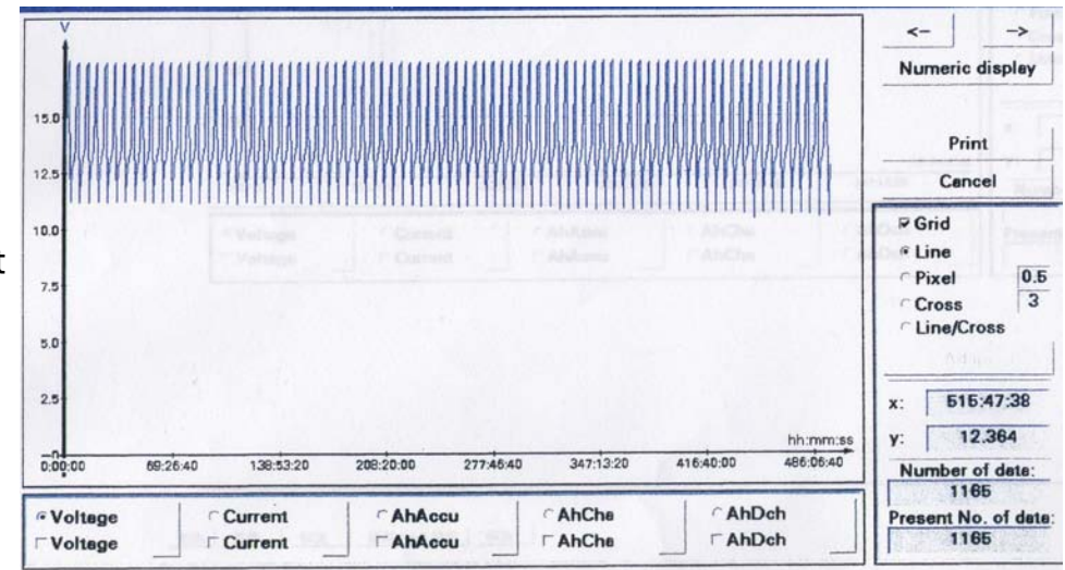
New battery #2 WITH SRS lasts 1320 hours (220cycles) This tests data chart has recorded 1165 hours (194 cycles)
