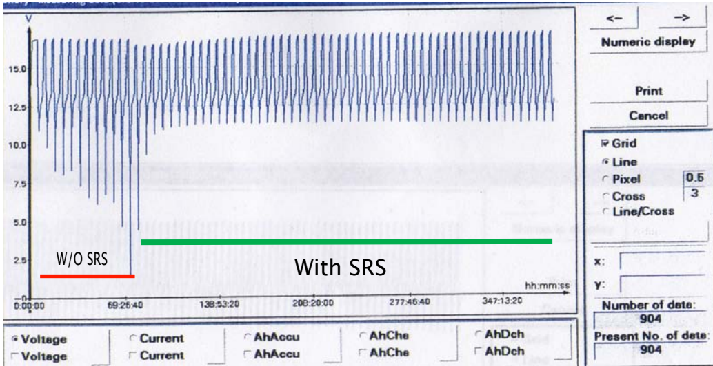
New Battery #1 W/O SRS Drops to 1.25V after approximately 69.26 hours. (11.5 cycles) SRS added at 11.5 Cycles. 99% recovery @ 14 cycles Was told battery lasted over 1,200 hours (200 cycles)
